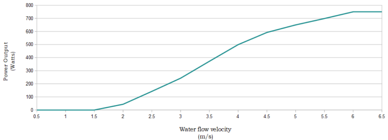
Hermetically sealed Generator Power Output Chart
